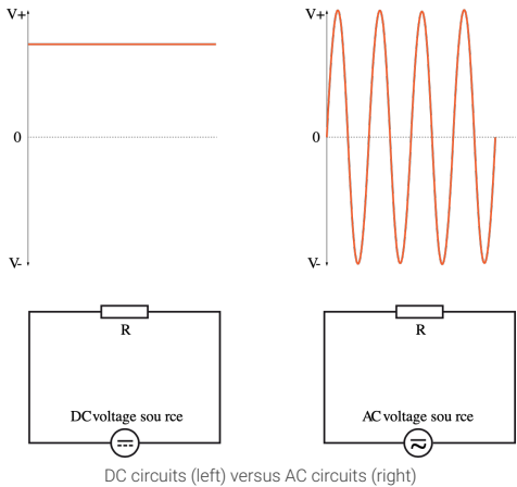
DC circuits (left) versus AC circuits (right)
