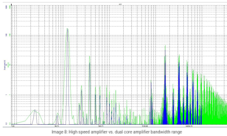
Image 8: High speed amplifier vs. dual core amplifier bandwidth range
