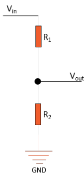
Image 15: Simple resistor voltage probe with the serial connection of two resistors
