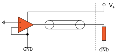
Image 13: Schematic illustration of a active voltage probe
