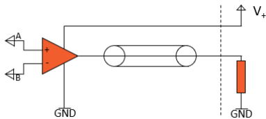
Image 14: Schematic illustration of a differential voltage probe
